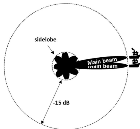
Figure 4-3 Azimuth resolution. Left radar screen, right targets and antenna beams. Please note that this is a simplification of real situations in which two ships will have unequal radar cross sections.
